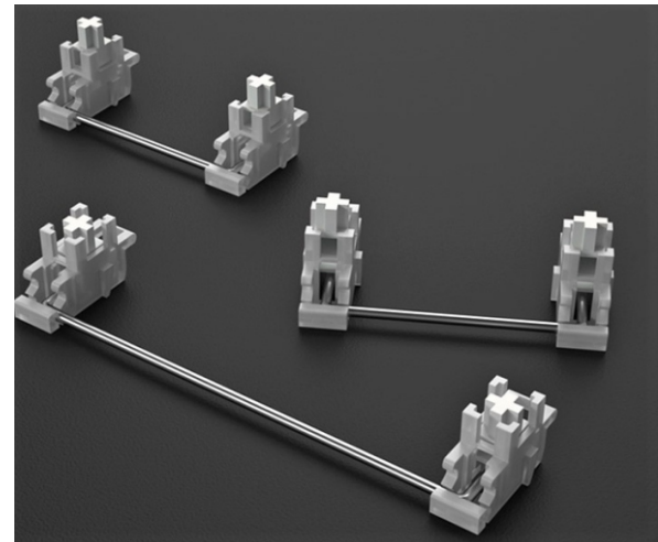
Satellite Axis /Balancing Axle
