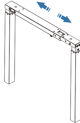
Desk frame with retractable length reduces the volume of out box and increases the qty of containers
